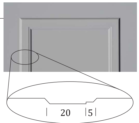
Groove Profile
